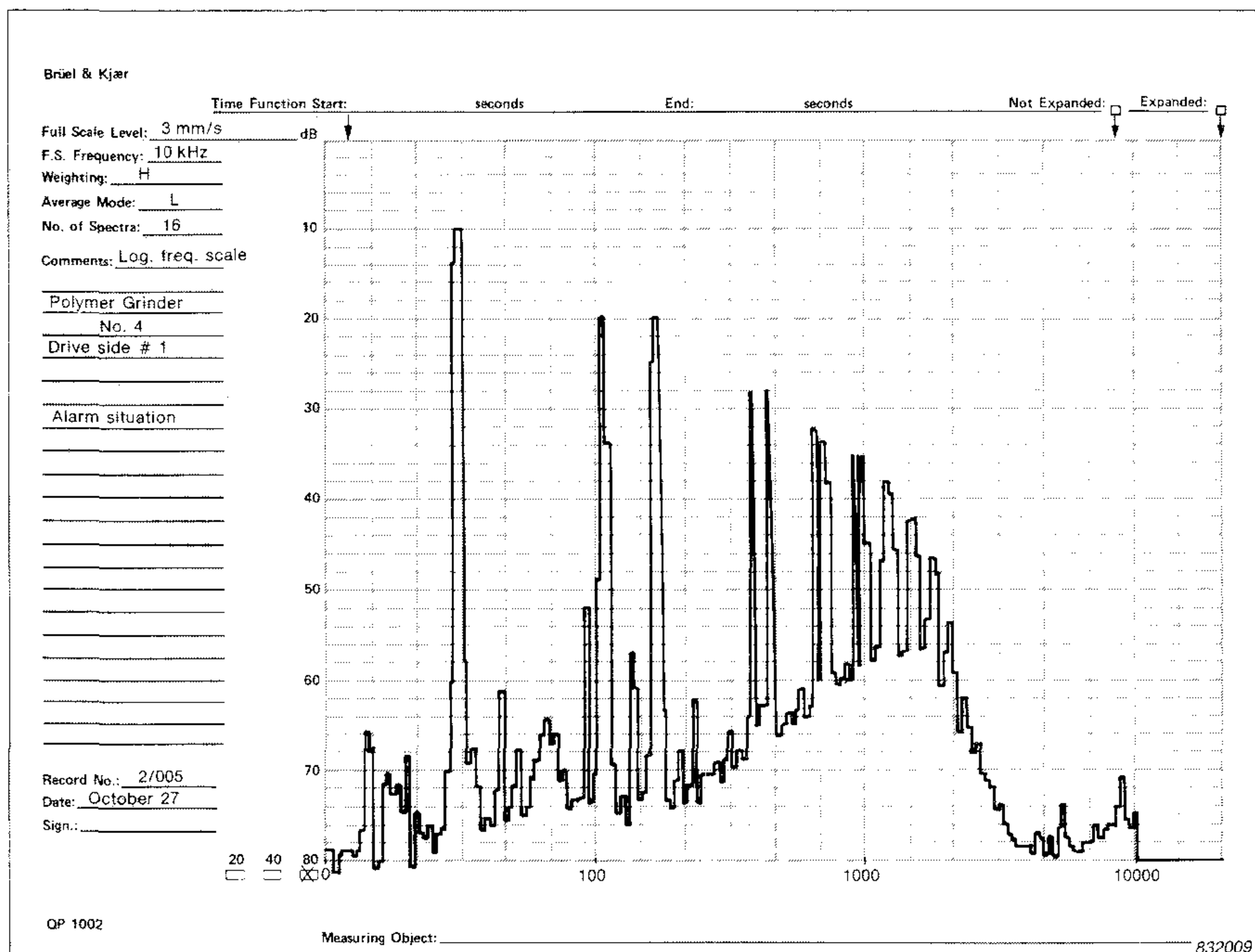
Fig. 4. New spectrum. Compared to Fig.2, there is an increase in amplitudes between 170Hz and 2000Hz
