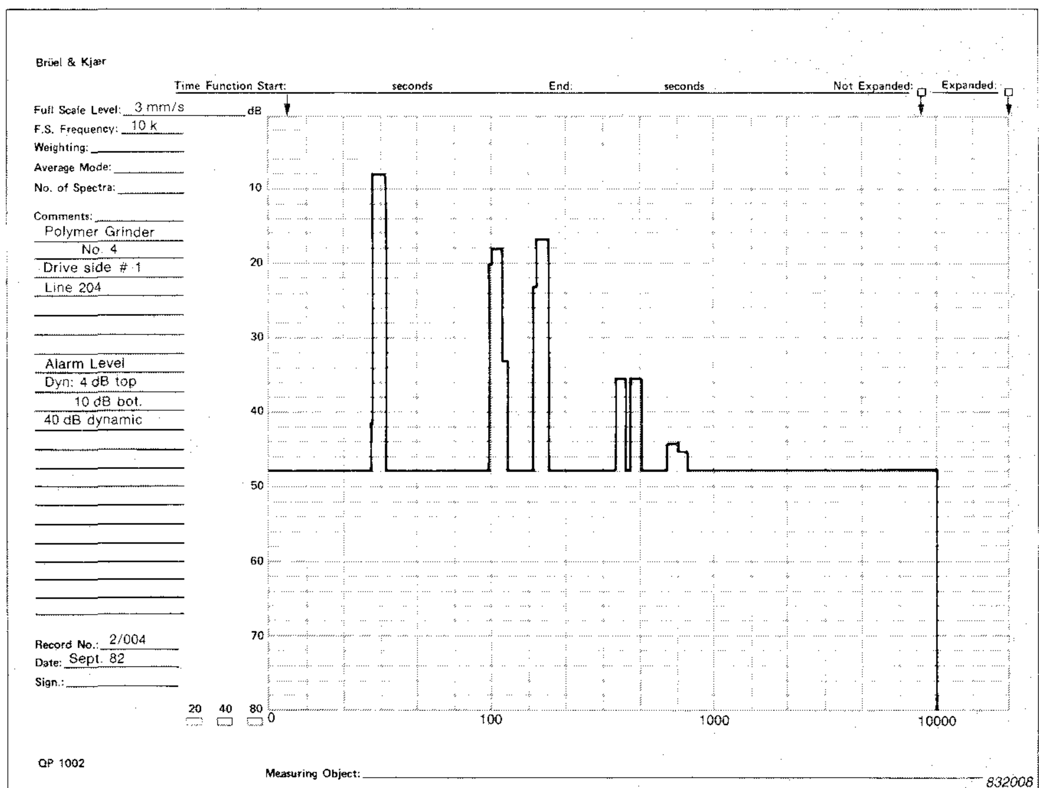
Fig. 3. Alarm levels calculated from the spectrum of Fig.2.
