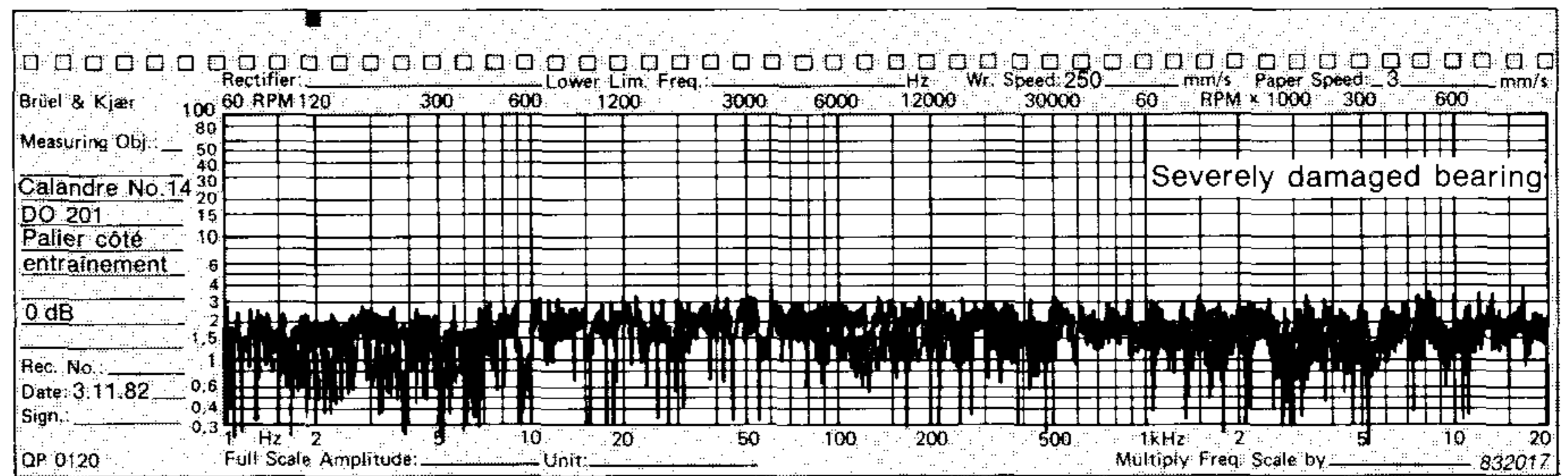
Fig. 6. SPM measurements on bearings at low frequencies
