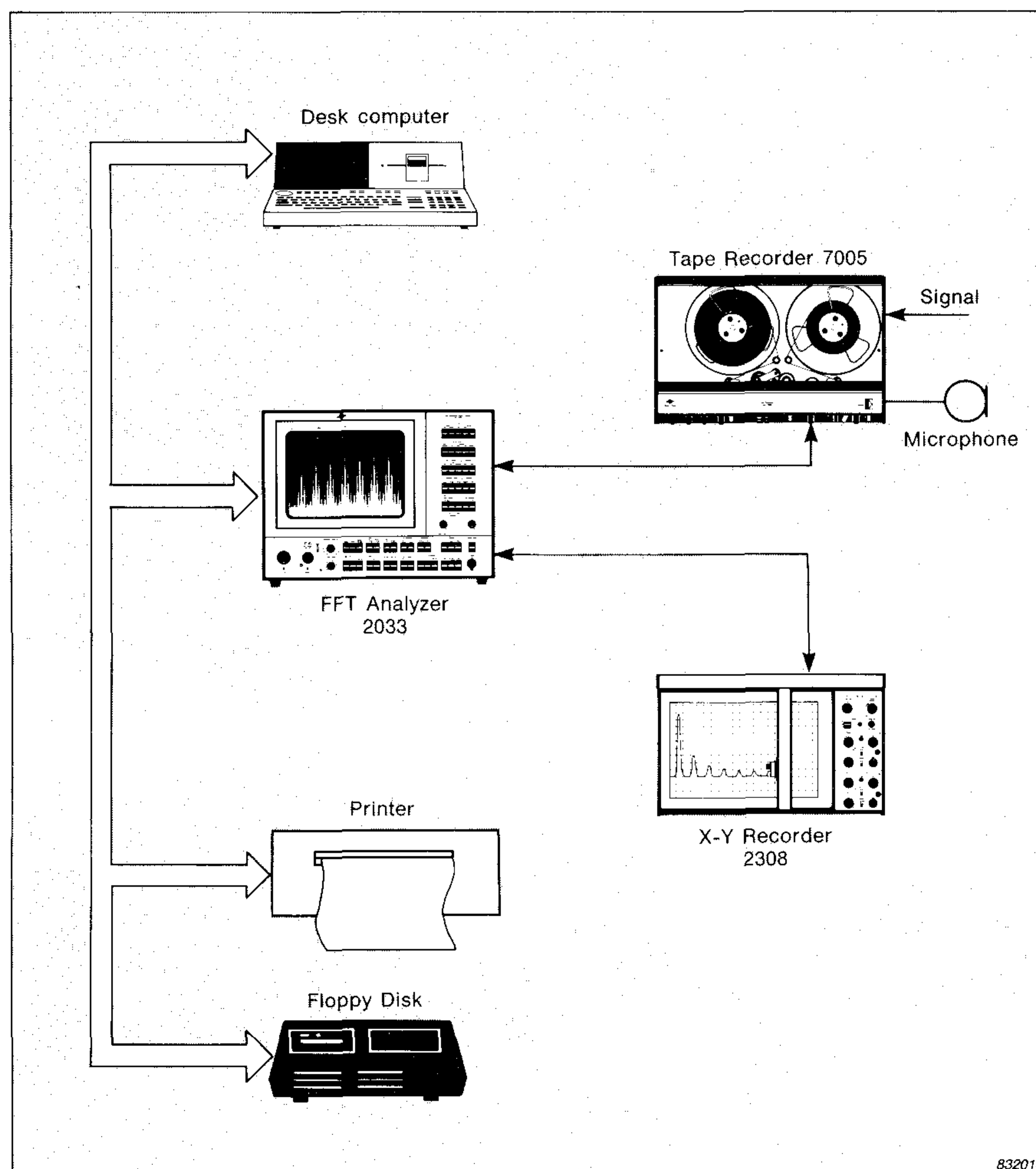
Fig. 1. Measurement system (phase 2)
