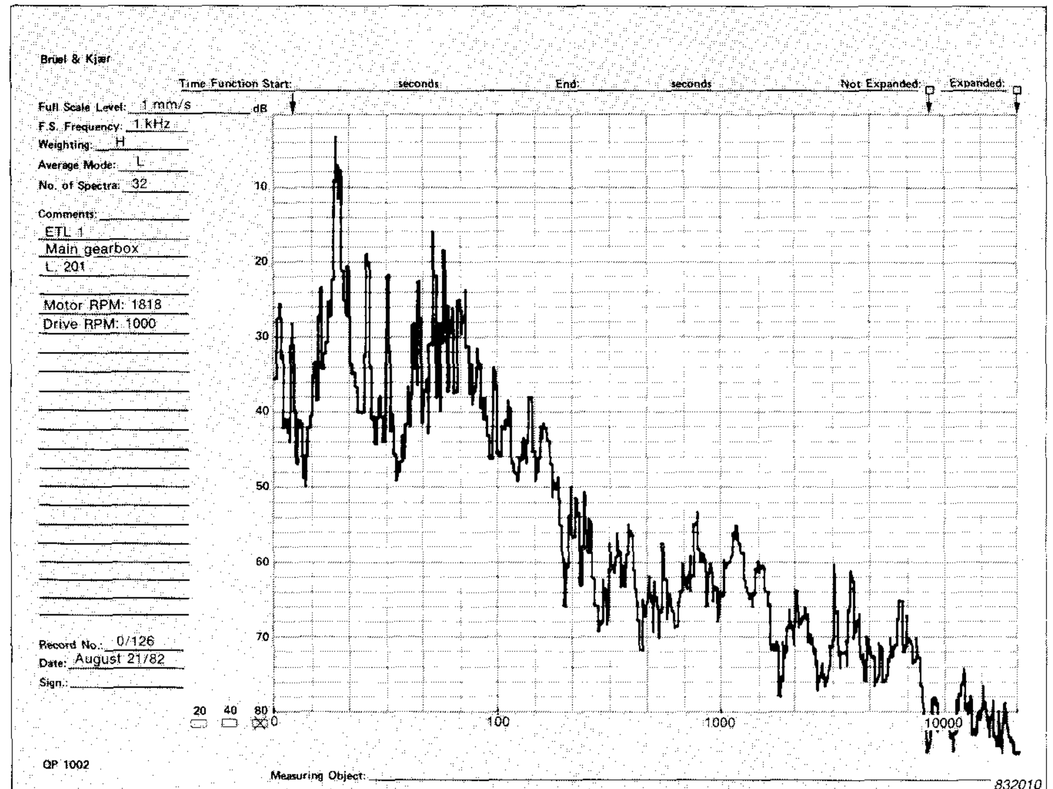
Fig. 8. Spectrum of a gear containing numerous harmonics and sidebands about the meshing frequency
