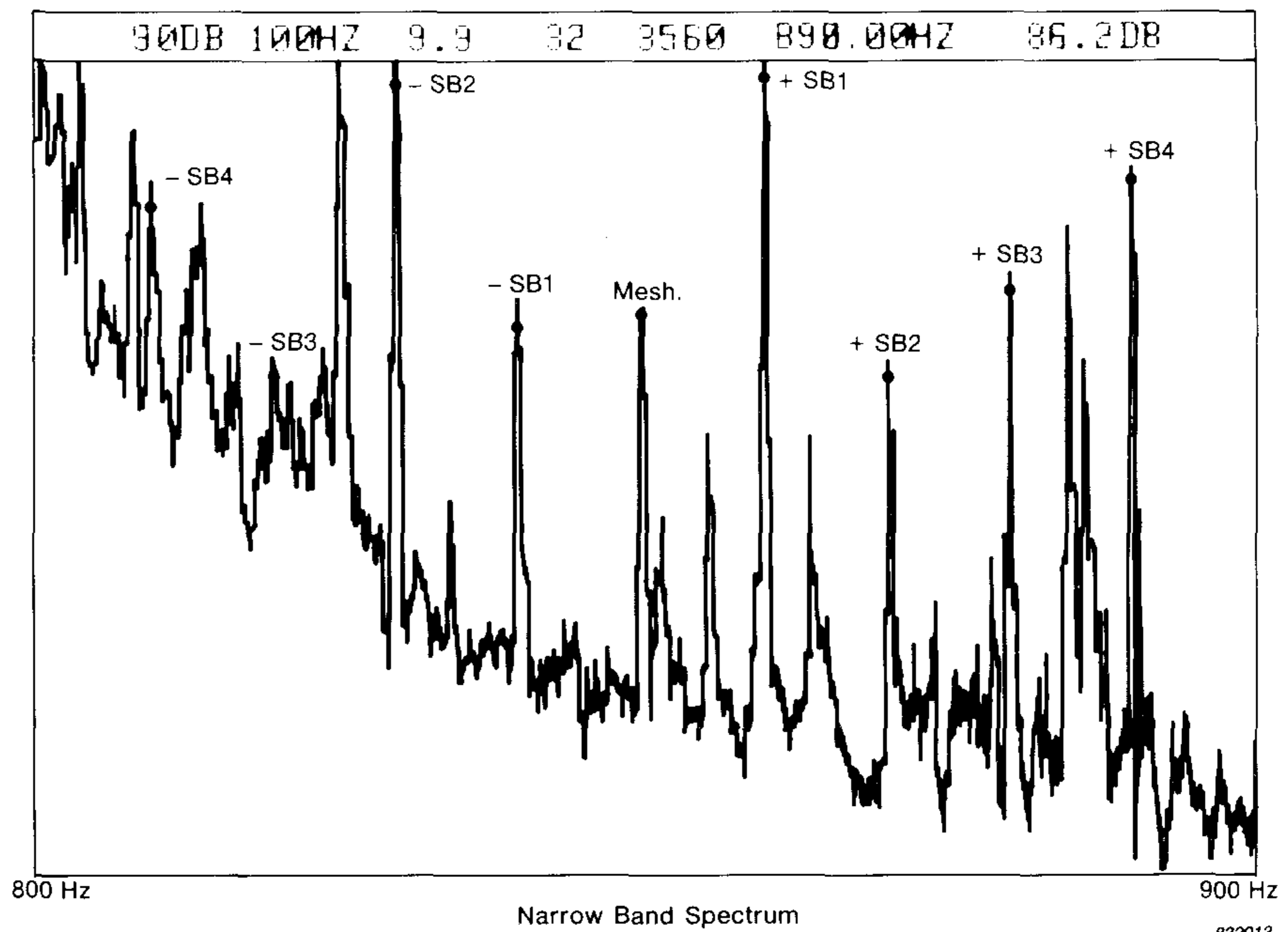
Fig. 7. Zoom of 100Hz about the meshing frequency of 850Hz showing the sidebands
